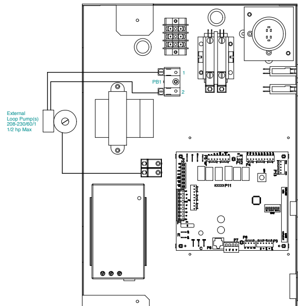
Figure 14: Pump Wiring 208-230/60/1
