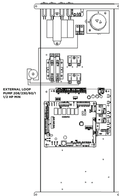
Figure 5: Source Pump Wiring 208-230/60/1
